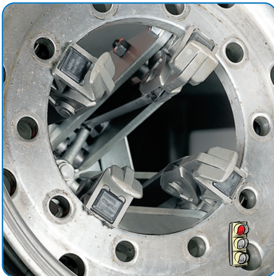
➤ Incorrect clamping procedure. Direct contact with clamp. Rim damage guaranteed
