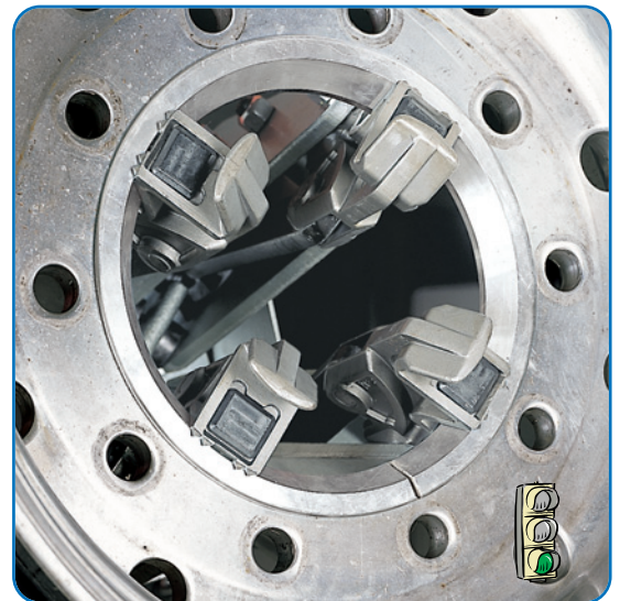
➤ Correct clamping procedure with ring. No direct contact between rim and clamp. Rim has maximum protection
